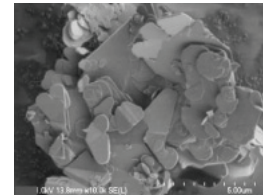
Scanning Electron Micrograph Grade ZG 10000X
